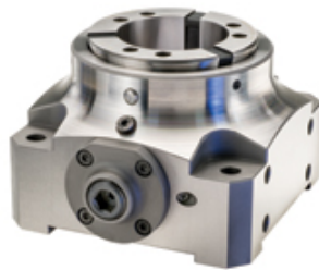
External Part Gripping Manual Actuation
